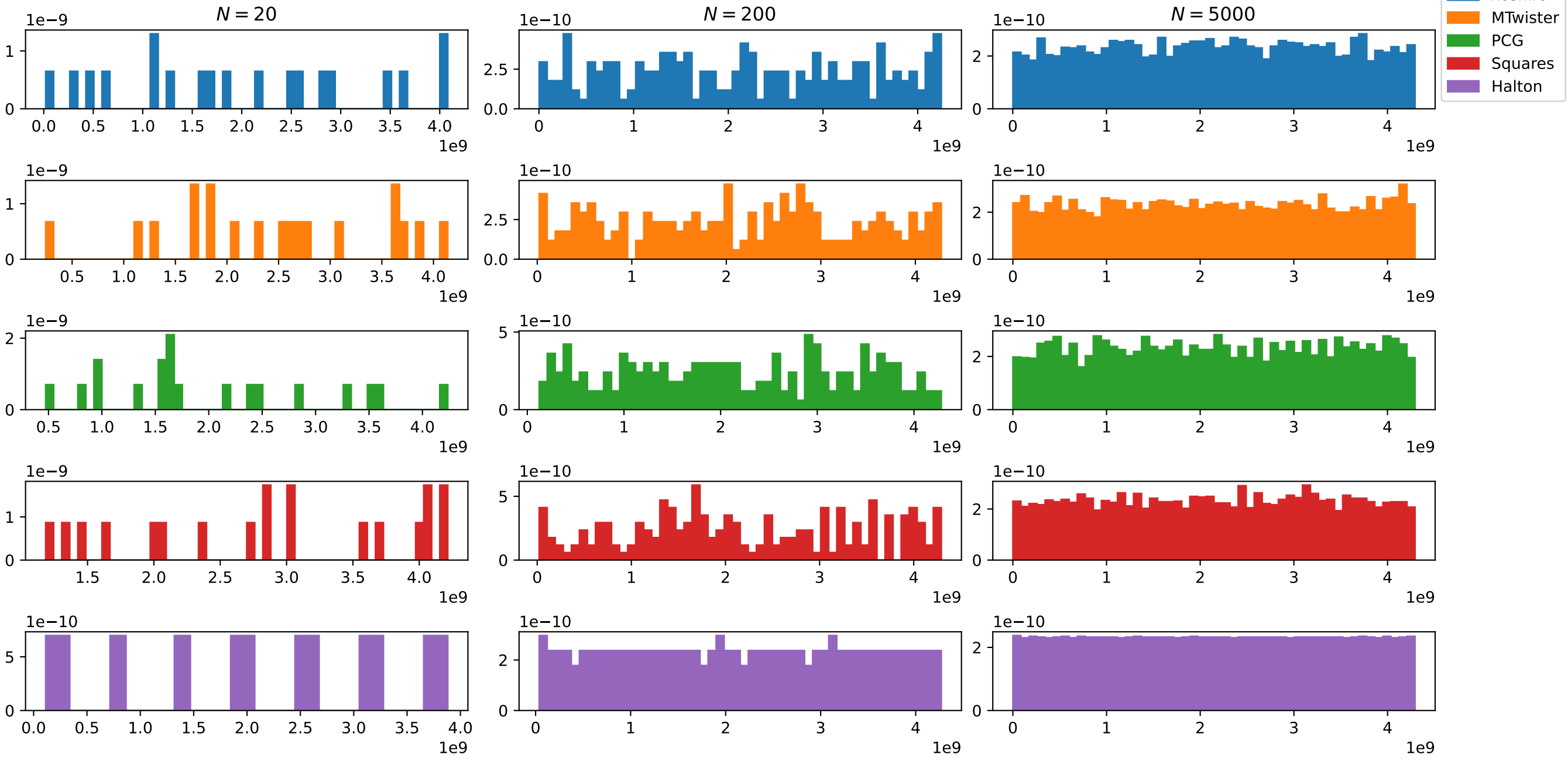
Histogram of different PRNG for different number of samples
