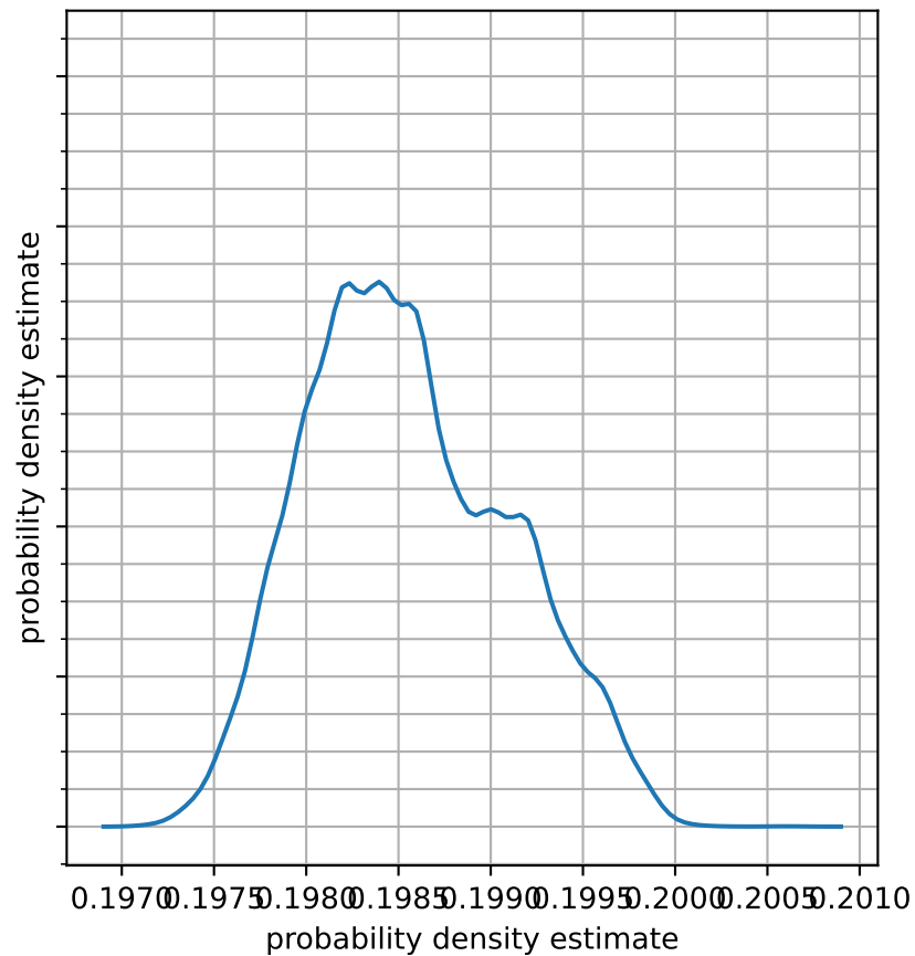
Float divide mean= 0.198\mu s
