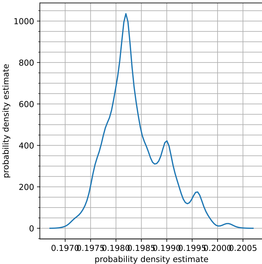
Float multiply mean= 0.198\mu s
