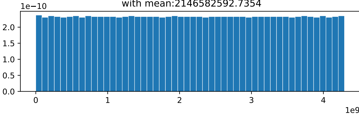
Histogram of Halton Sequence with mean:2146582592.7354
