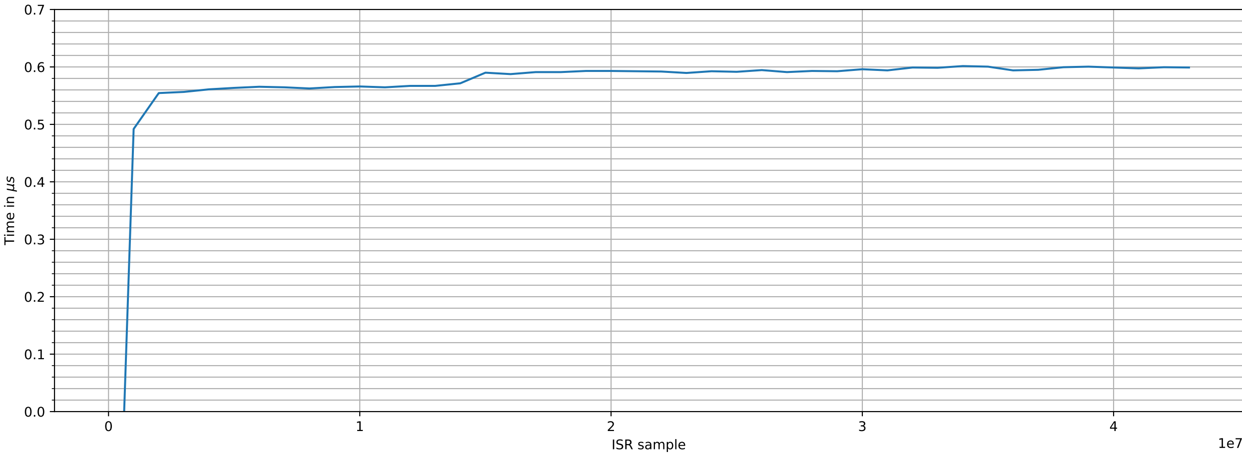
Execution time to generate one random uint32_t
