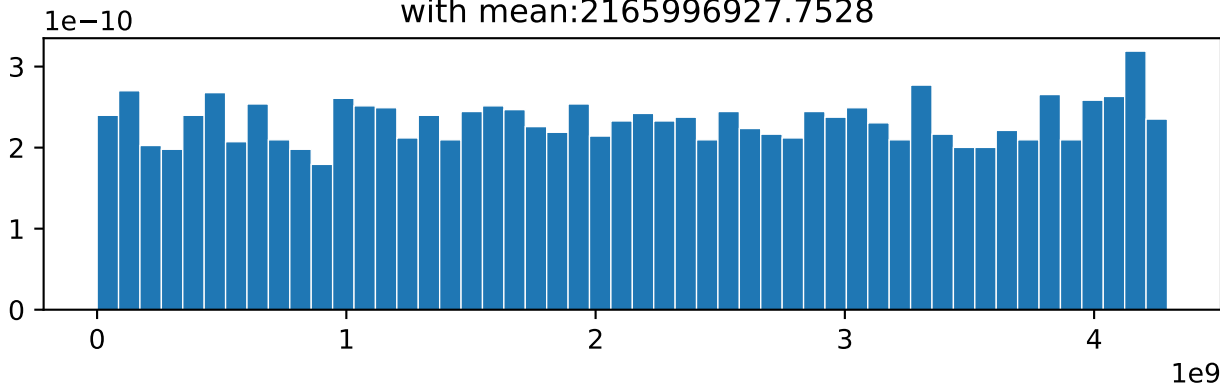
Histogram of MTwister with mean:2165996927.7528
